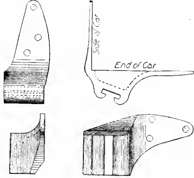
Figs 3348-3351 Bracket for Tail-lamp.
